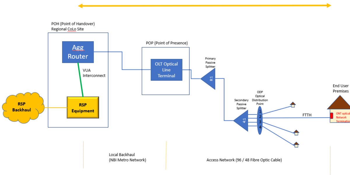
Figure 2: Overview of the Wholesale VUA solution architecture
