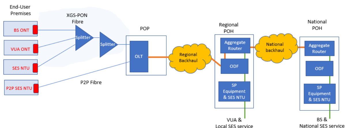
Figure 11: Fibre Access to Aggregation Models
