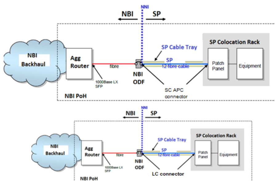
Figure 10: InterConnect In-Building Handover (IBH)
