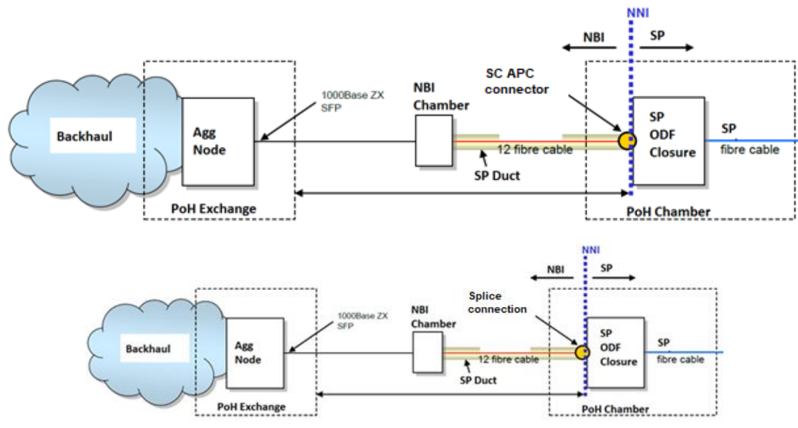
Figure 9: InterConnect In-Span Handover (ISH)
